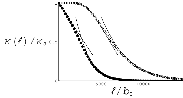
Fig. 1 – Renormalized bending rigidity \kappa(\ell)/\kappa_0 as a function of the length scale \ell/b_0 = 2^N for K_0 = 1000 for d = 2 ( \circ ) and d = 3 ( \bullet ) according to the recursion relation (17). The lines show the asymptotic behavior for \ell \gg \kappa_0/T and \ell \ll \kappa_0/T according to eqs. (18) and (20), respectively.
